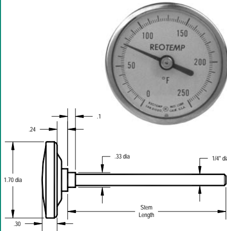
Model G - 1 11/16" Dial
